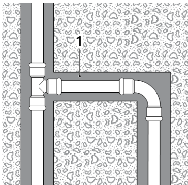
Figure 6: Concealed pipe
