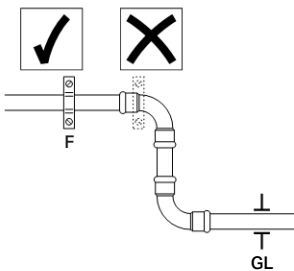
Figure 44: Positioning anchor points: On the pipe, not on the pressfitting
