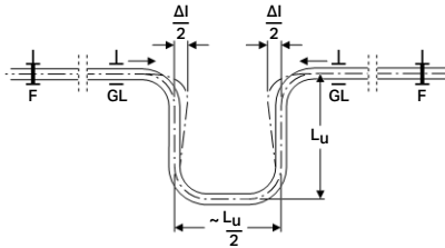
Figure 23: U-bend expansion compensation from bent pipe
